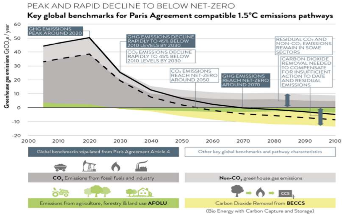
Figure 1. Illustration of the three benchmarks in Paris Agreement Article 4.1 for operationalisation of Article 2.1 (dark blue boxes) and global decarbonisation benchmarks (white box). This representative pathway is the median across all 1.5°C-compatible pathways from the IPCC SR15 that reach levels of Carbon Dioxide Removal (CDR) below the upper end of estimates for sustainable, technical and economic potential around 2050 from SR15 in the sector of Agriculture, Forestry and Land-Use (AFOLU), as well as via Bioenergy combined with Carbon Capture and Storage (BECCS) 9 .
